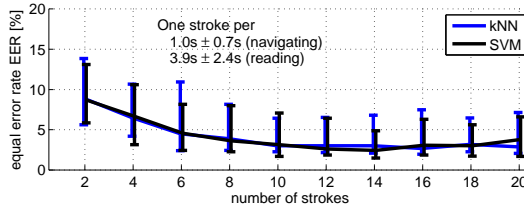
Figure 5: The equal error rate (ERR) as a function of the number of strokes taken for one classifier decision. The error converges at 11 to 13 strokes. For the first decision, the system must wait until all required strokes have been recorded. For all subsequent decisions, a sliding window of past strokes will be taken such that a new decision can be made at every other stroke.
